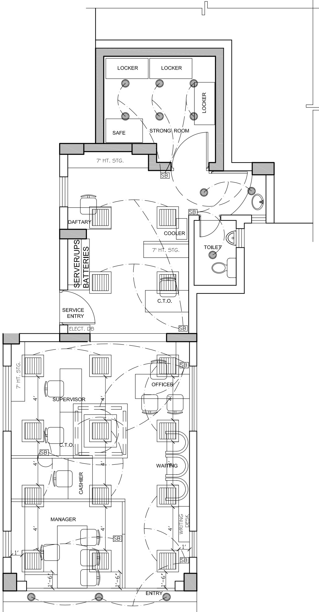
REFLECTED CEILING PLAN AT MIRA ROAD.
