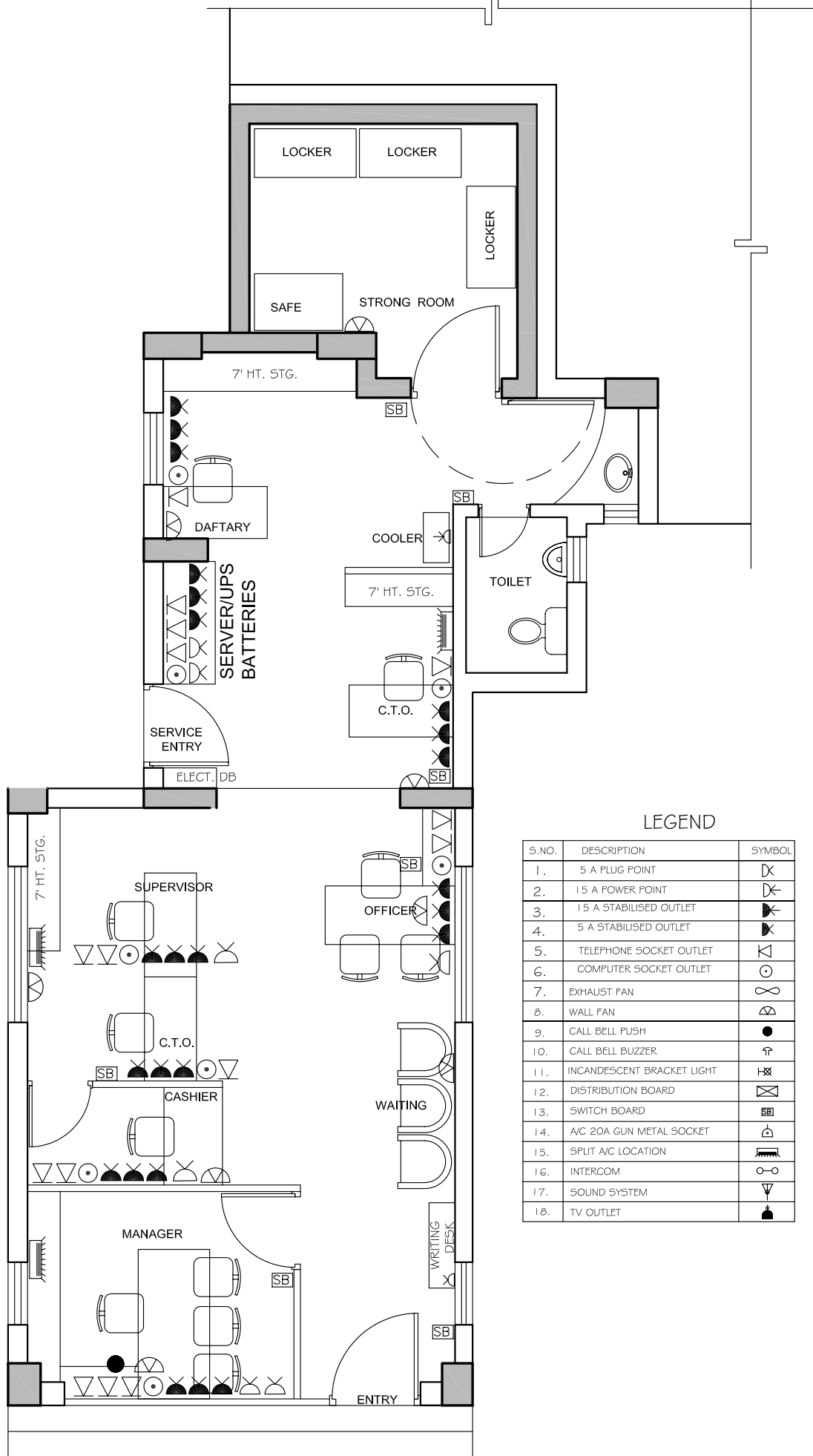
ELECTRICAL PLAN AT MIRA ROAD.
